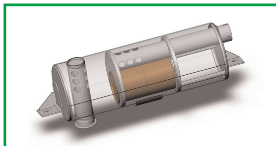
3D Image of the MINE-X® Catalytic Muffler
